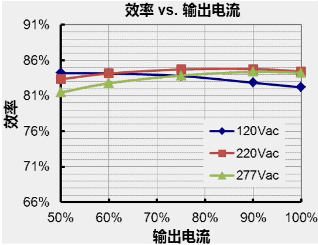
EUV-042S036PS 效率 vs. 输出电流
